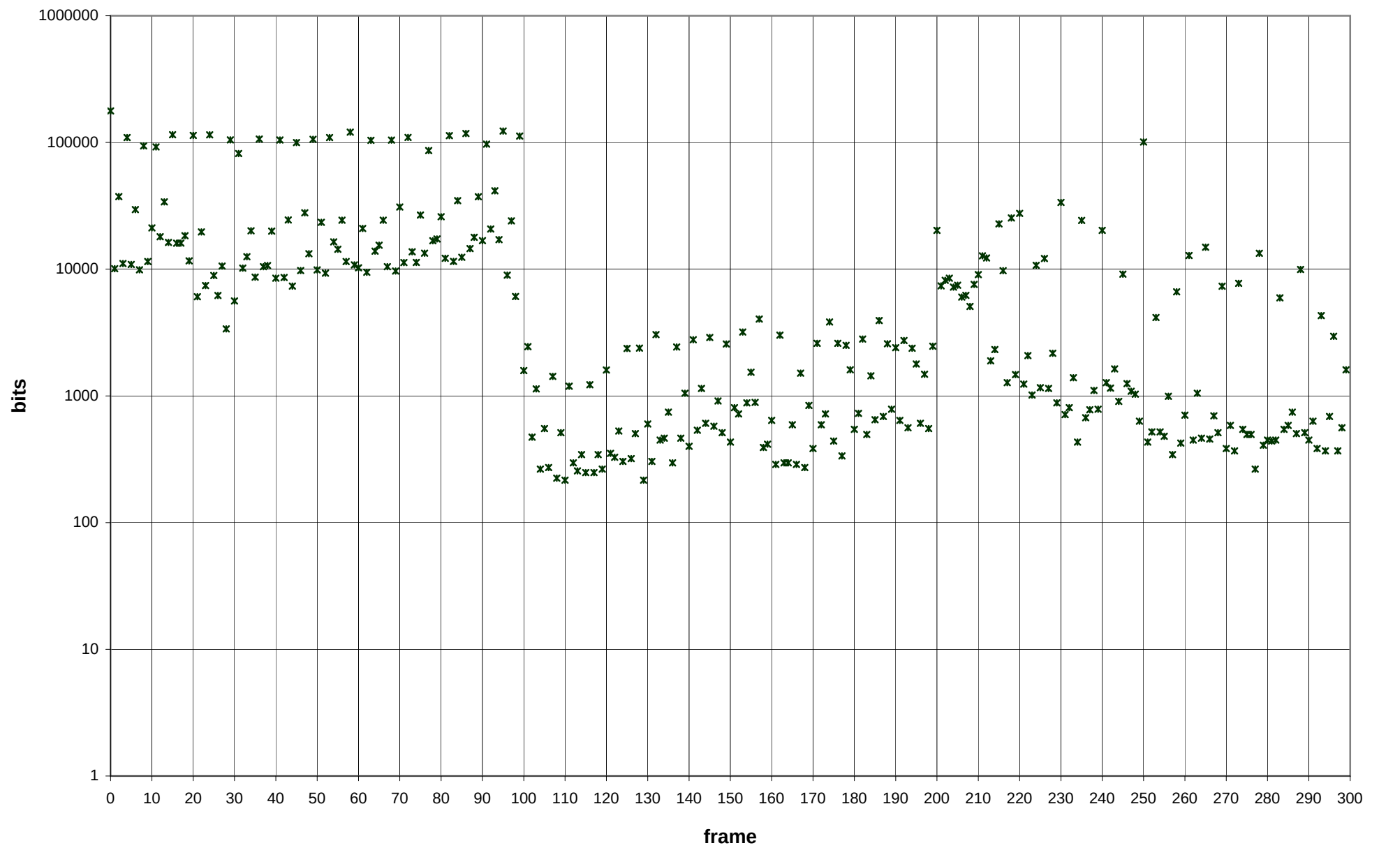
x265 with zones: bits per frame
