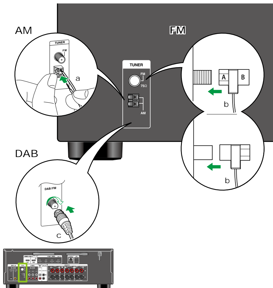
a AM loop antenna, b Indoor FM antenna, c DAB/FM antenna
