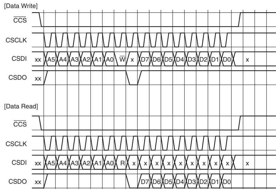
Figure 2-13. Serial Interface
