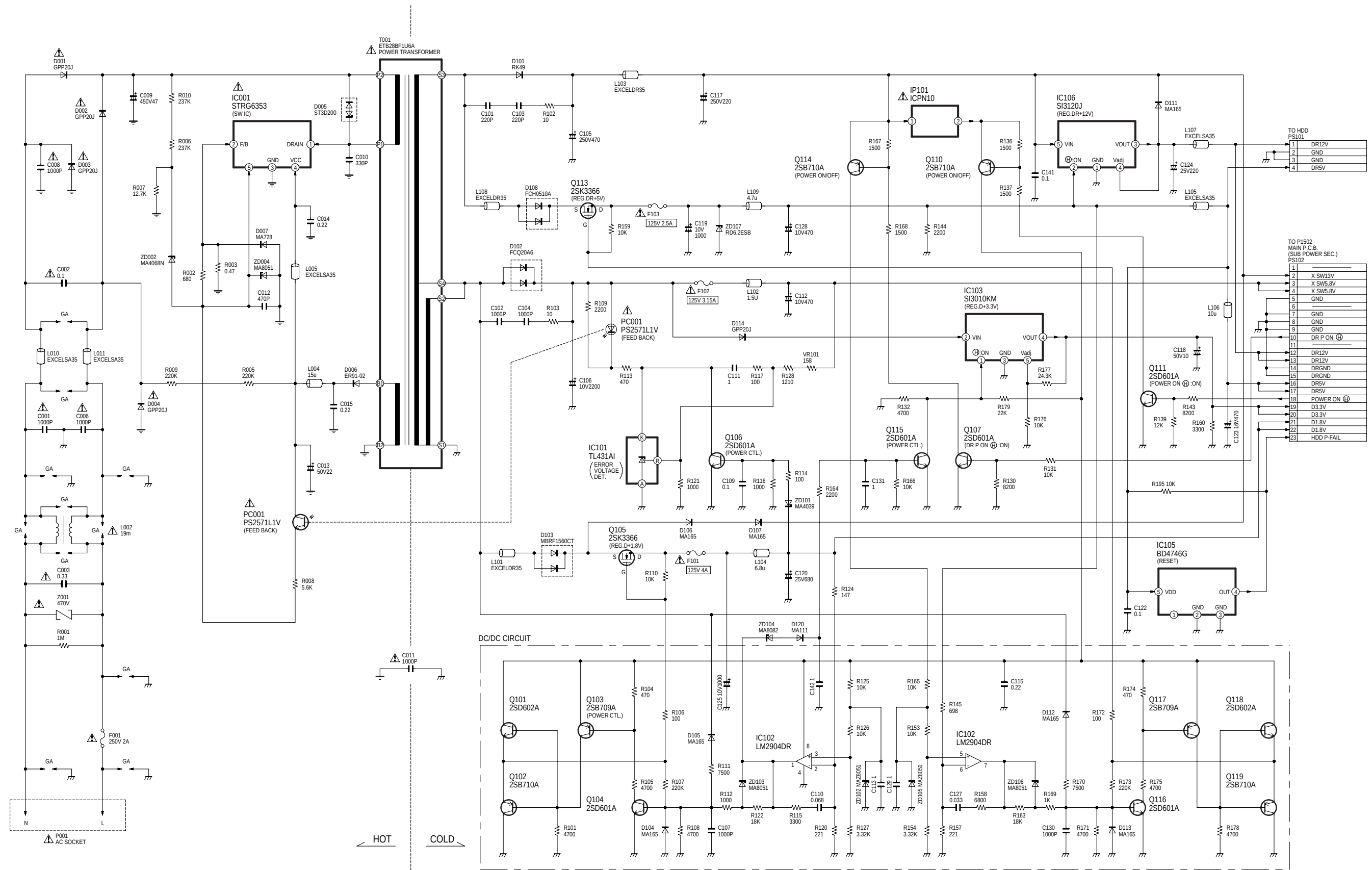
DMR-E85HEB/EG Main Power Supply Schematic Diagram
