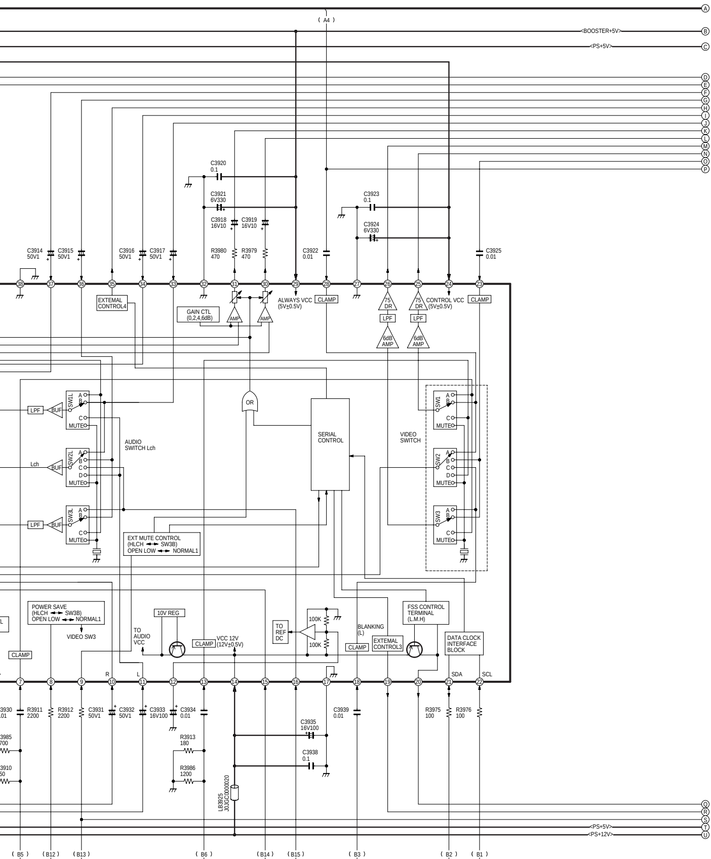
DMR-E85HEB/EG Scart Schematic Diagram
