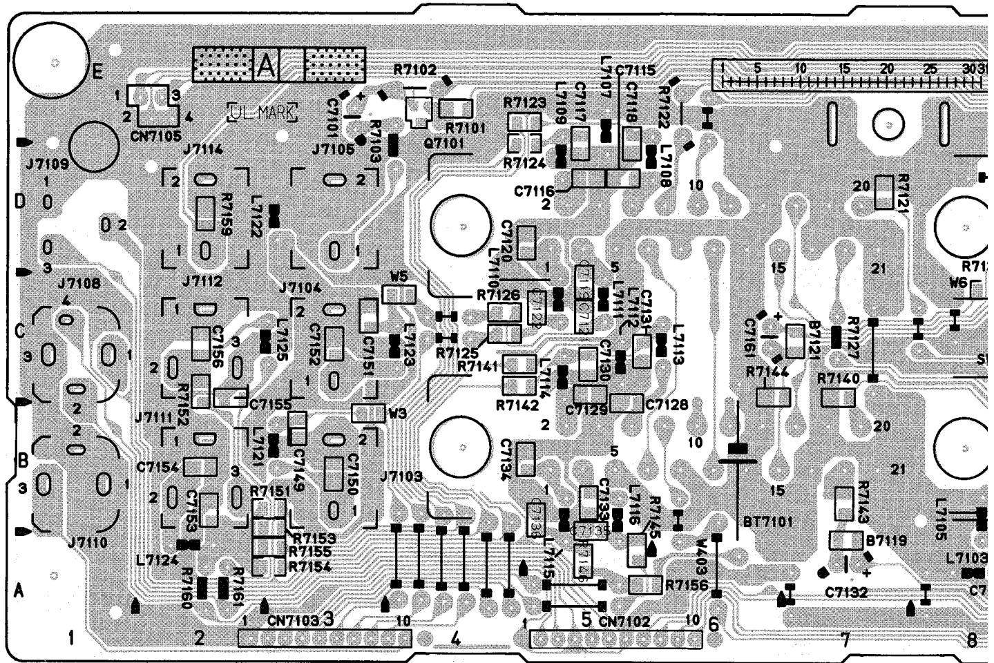
COMPONENT PARTS LOCATION GUIDE <TERMINAL>
