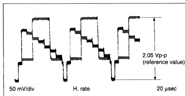
Fig. 3-3-8 D/A LEVEL
